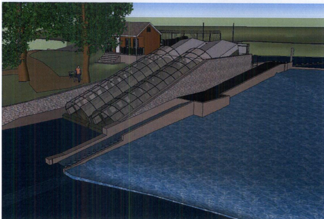
Figure 4: Design concept sketch to indicate scale, showing new fish pass adjacent
